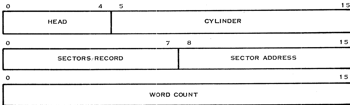
Figure 3-12. Header Data Format
