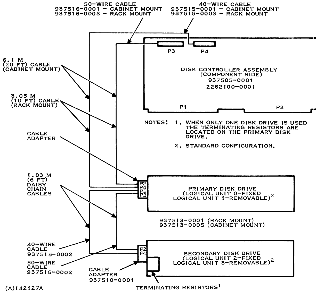
Figure 1-5. Interconnection of Disk Controller and Two Disk Drives
