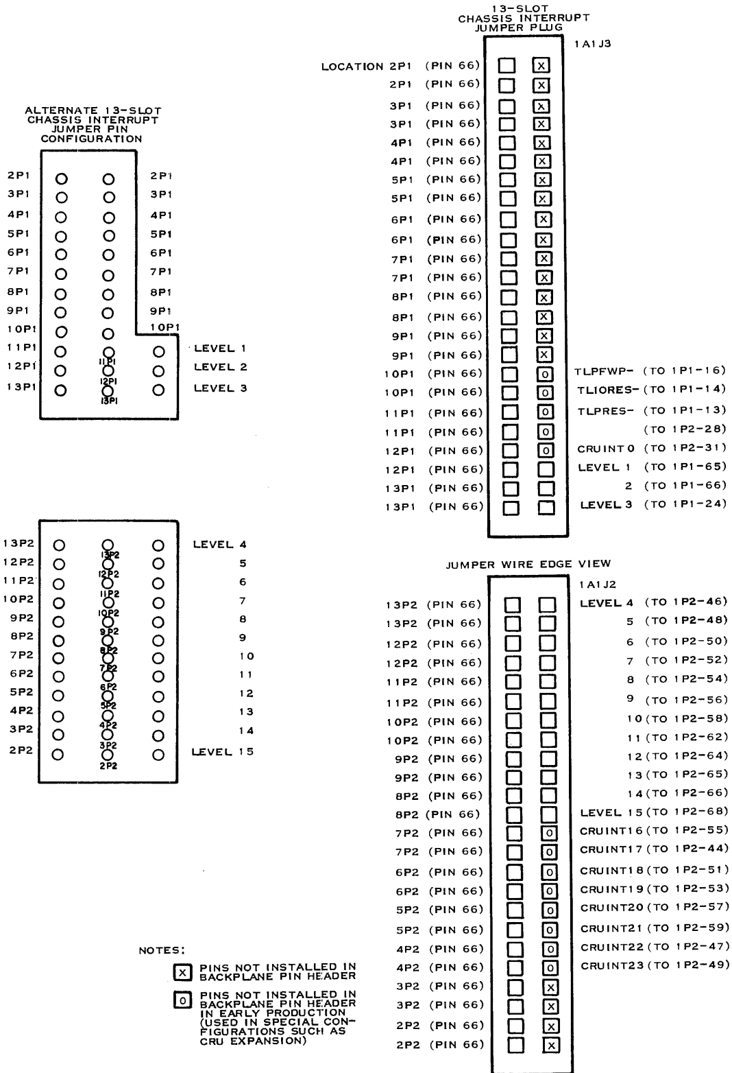
Figure 2-29. 13-Slot Chassis Interrupt Jumper Plugs
