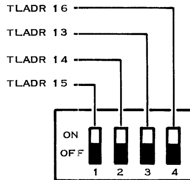
Figure 2-32. TILINE Slave Address Switches
