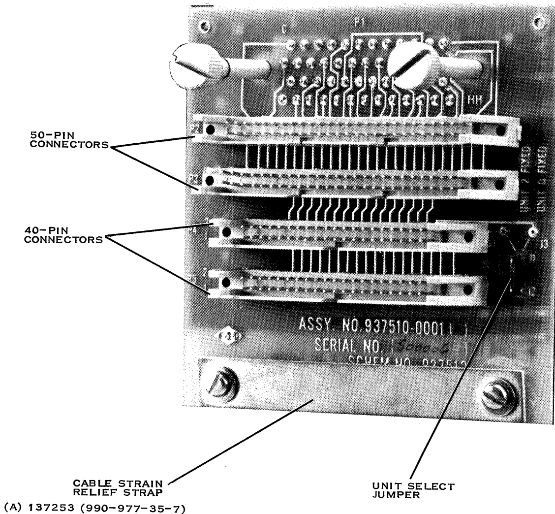
Figure 2-35. Cable Adapter
