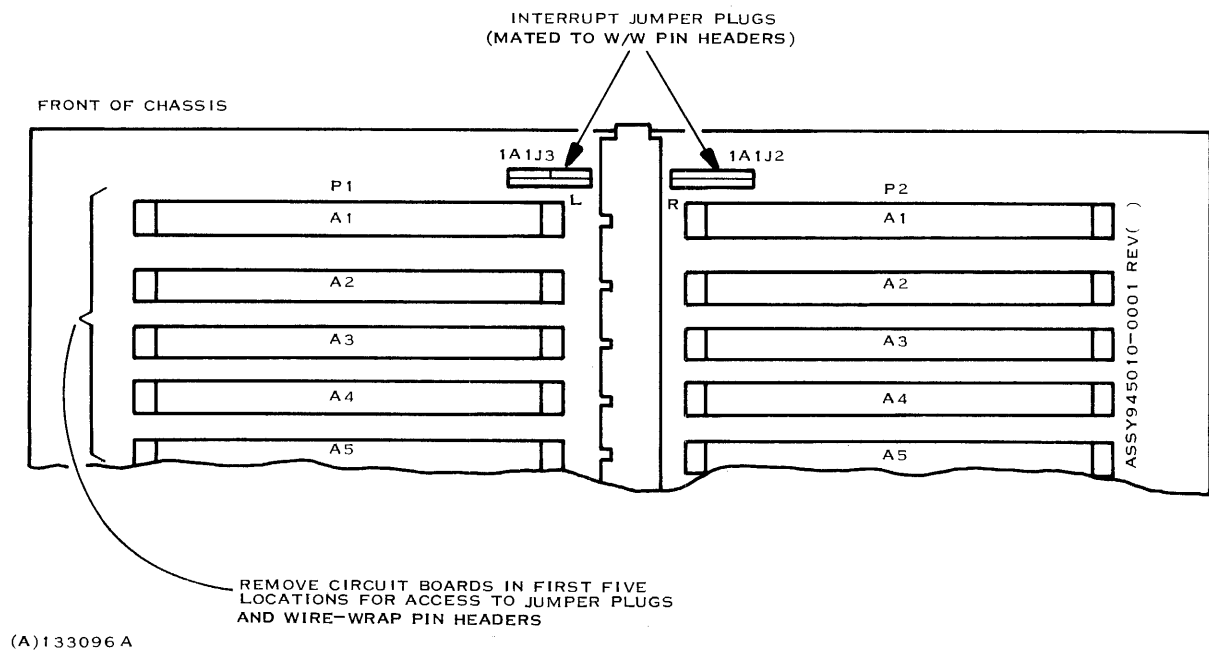
Figure 2-27. Location of Interrupt Jumpers (6- and 13-Slot Chassis)
