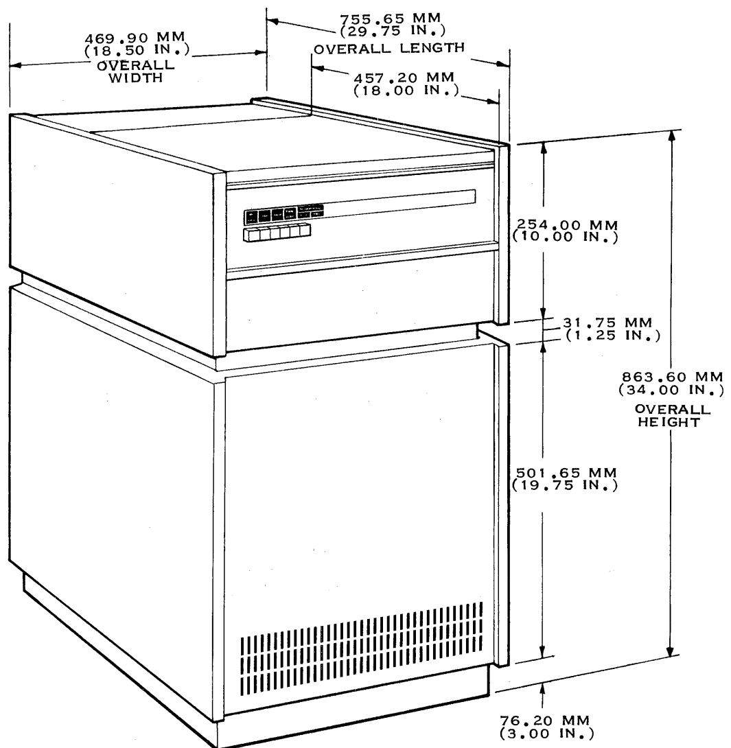
Figure 2-3. Physical Dimensions of Cabinet Mount Model DS10 Cartridge Disk Drive
