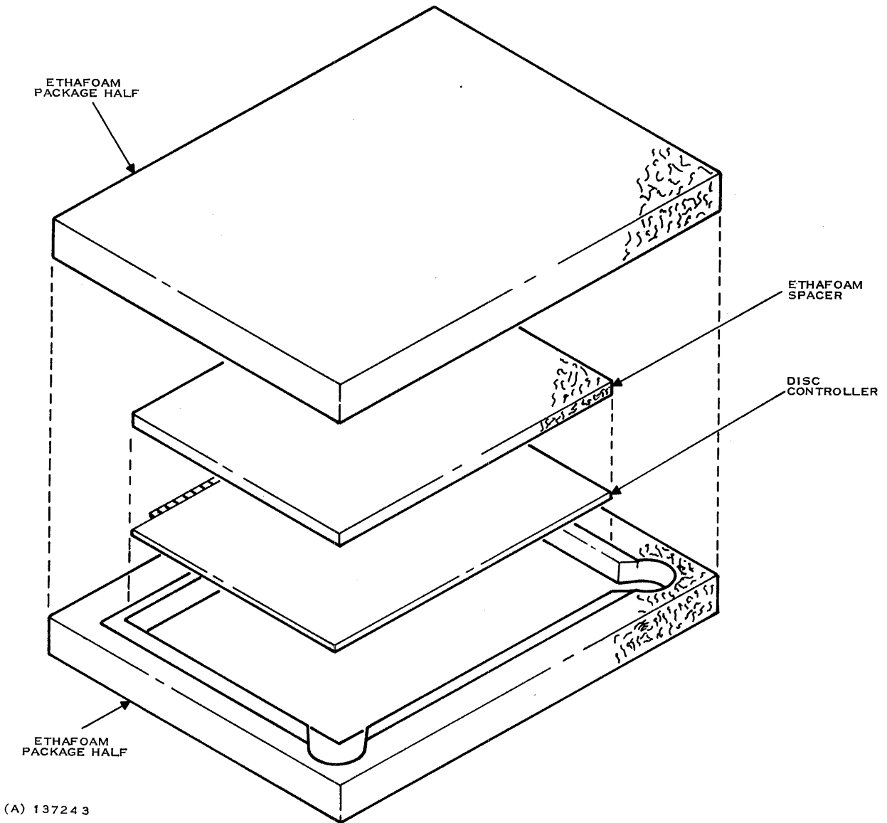
Figure 2-16. Disk Controller Shipping Configuration
