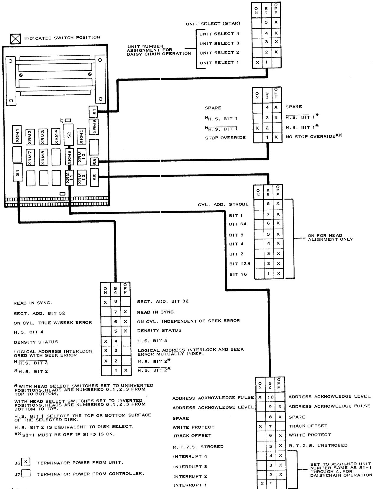
Figure 2-40. Switches and Settings for Cabinet Mount Primary Disk Drive
