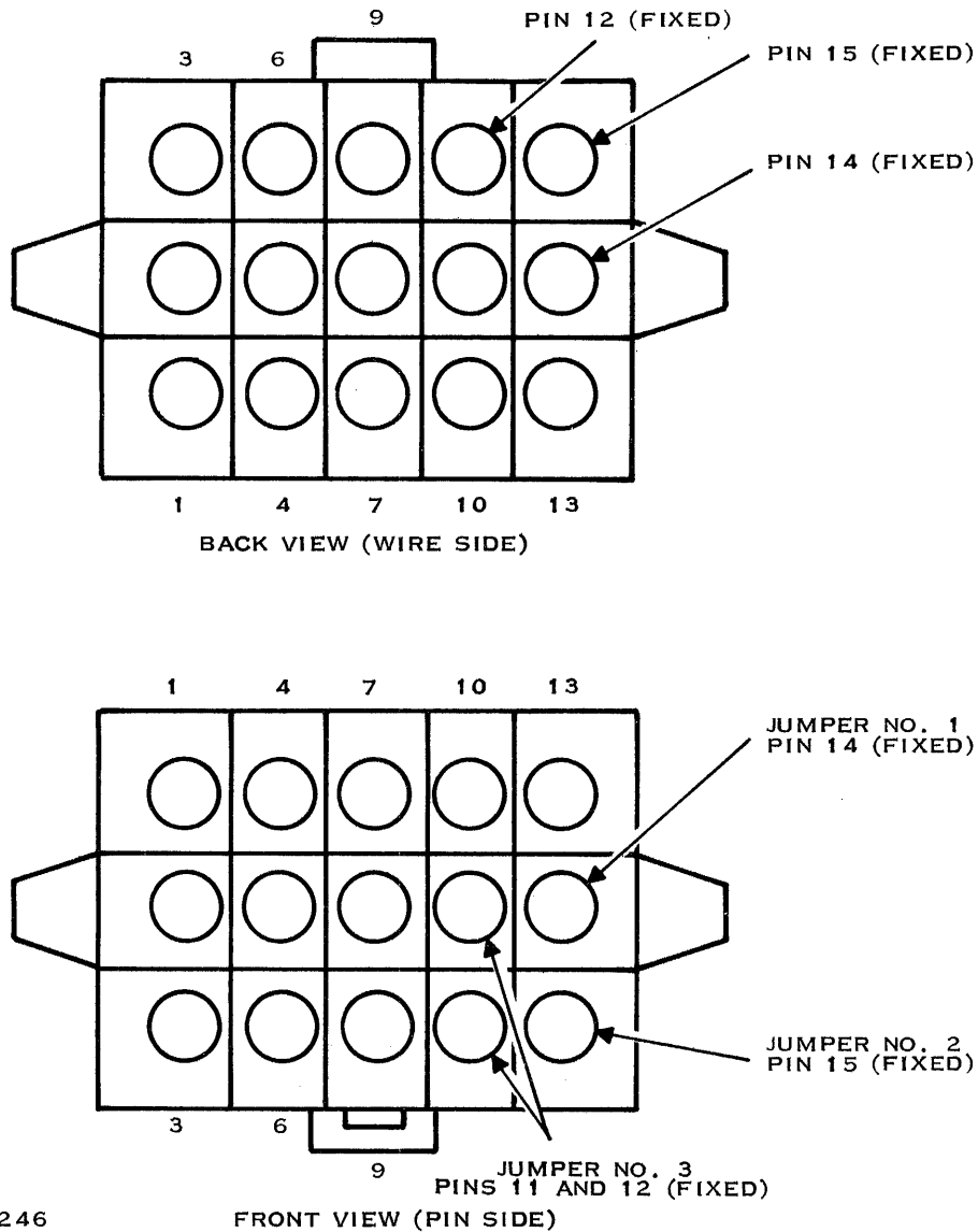
Figure 2-19. Voltage Jumper Plug and Connector
