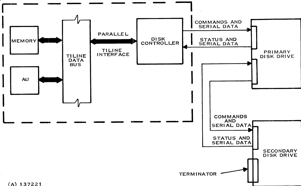
Figure 1-2. Model DS10 Cartridge Disk Unit Subsystem Simplified Diagram
