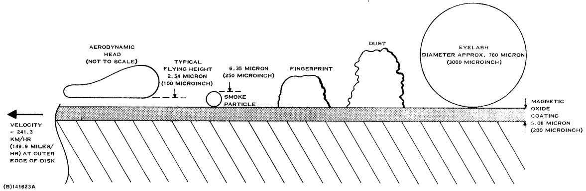
Figure 4-5. Disk Contaminants
