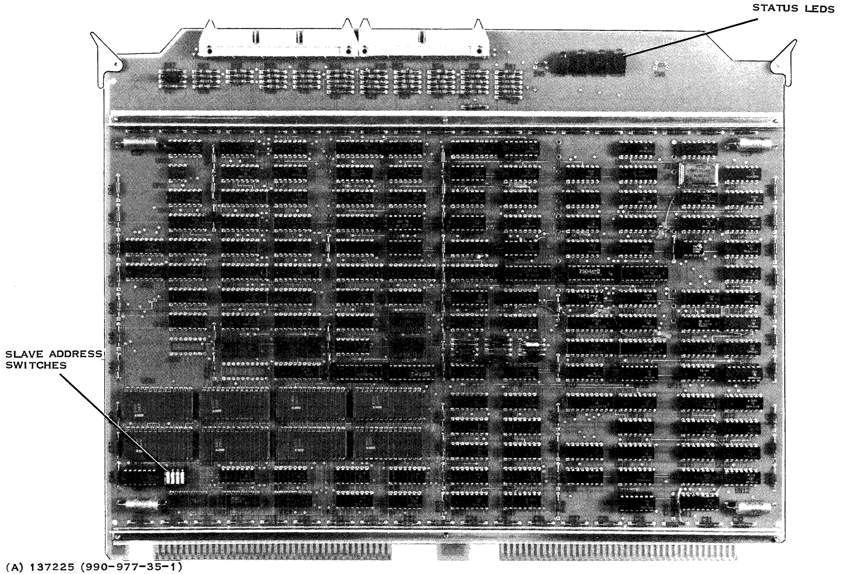
Figure 2-31. Model DS10 Cartridge Disk Controller (PWB)
