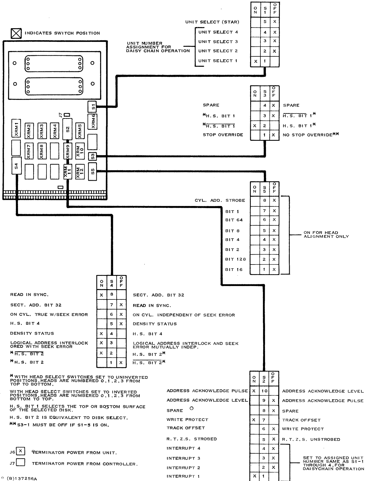
Figure 2-39. Switches and Settings for Rack Mount Primary Disk Drive
