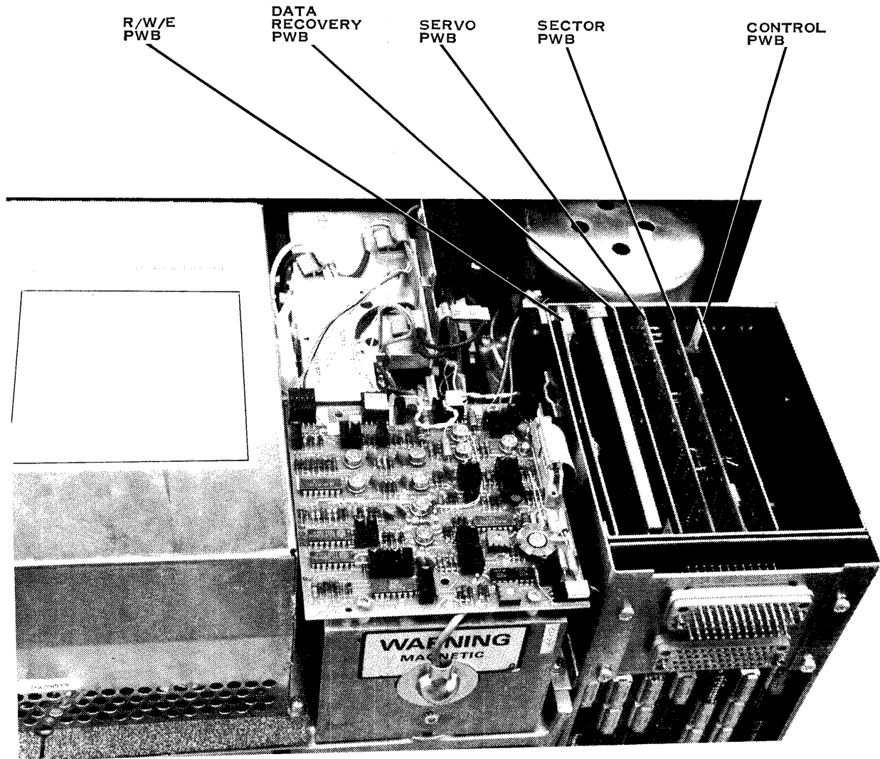
Figure 2-10. Disk Drive PWB Locations
