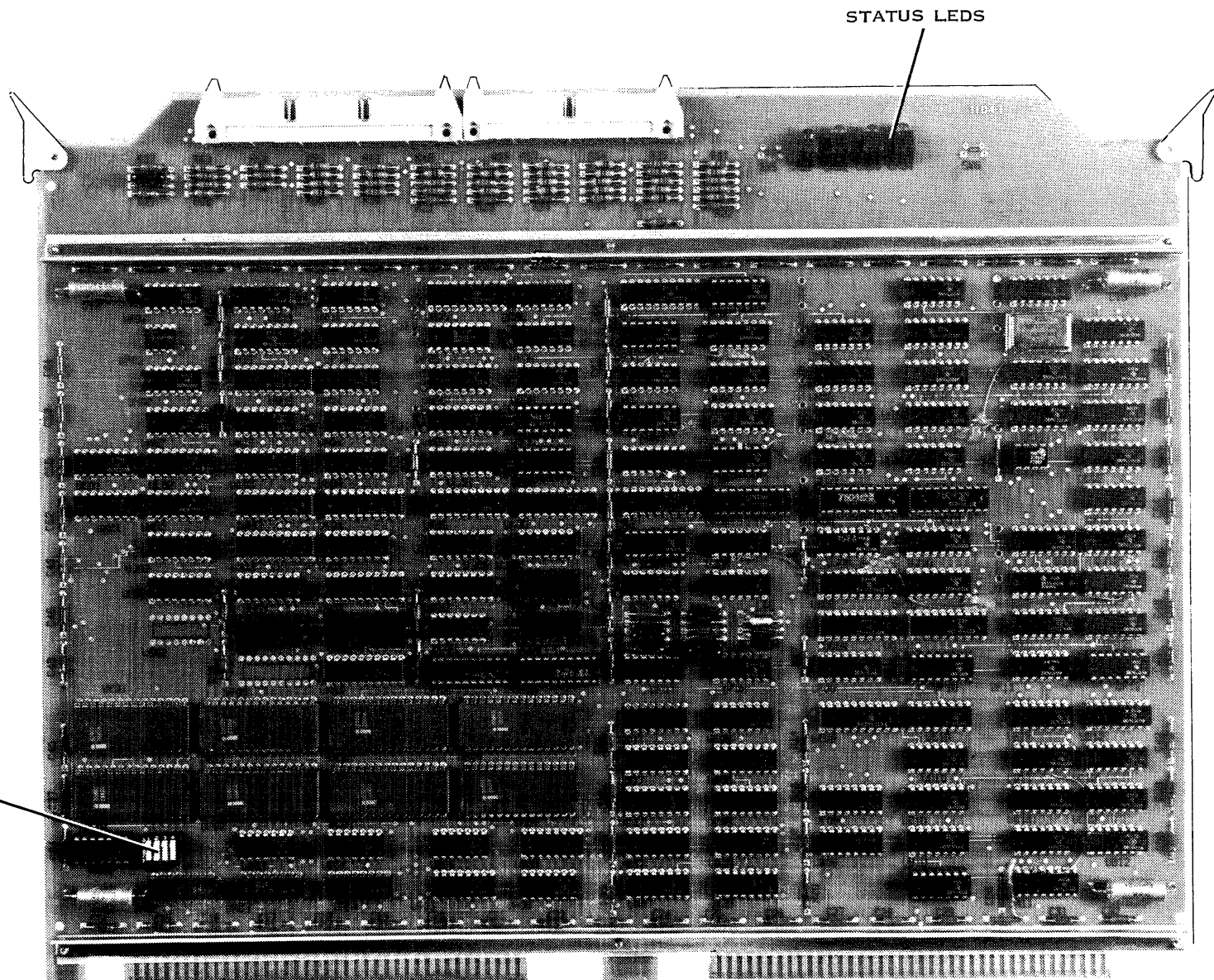
Figure 1-6. Model DS10 Cartridge Disk Controller (PWB)
